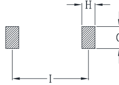
Suggested PWB Layout
